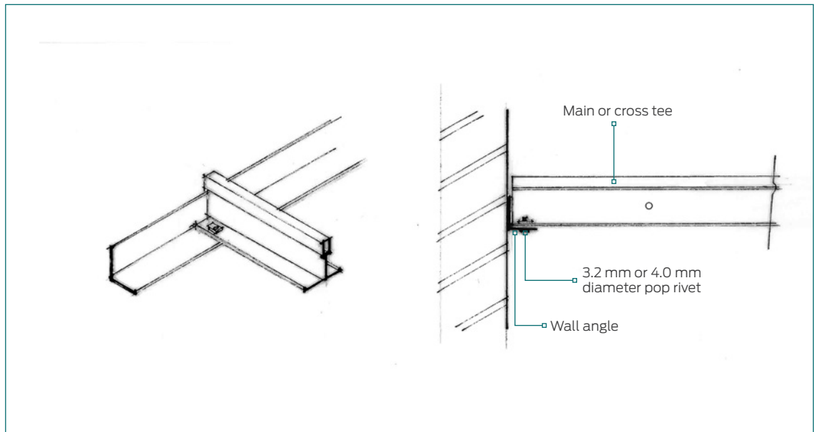
Figure 53: Pop rivet.
